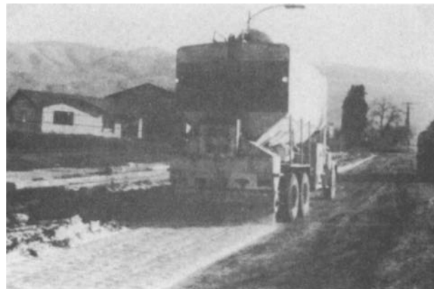
Figure 4-27. Distribution of quicklime from mechanical spreader on city street.
